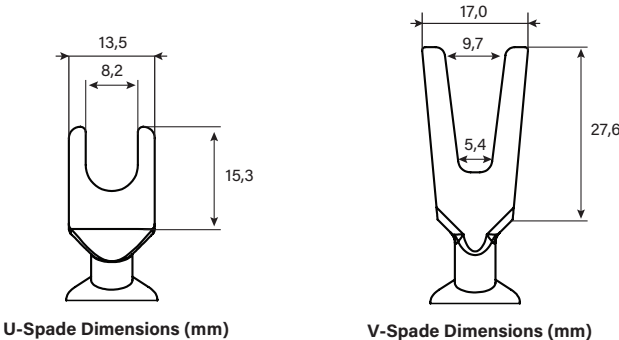
U-Spade Dimensions (mm)
