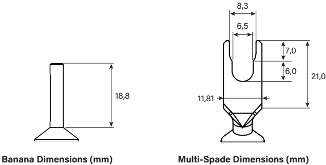
Banana Dimensions (mm)
